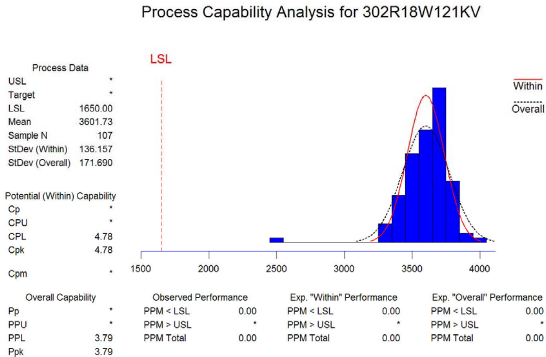
Figure 2. AC Breakdown Results for Test Lot of 302R18W121KV4 Capacitors
