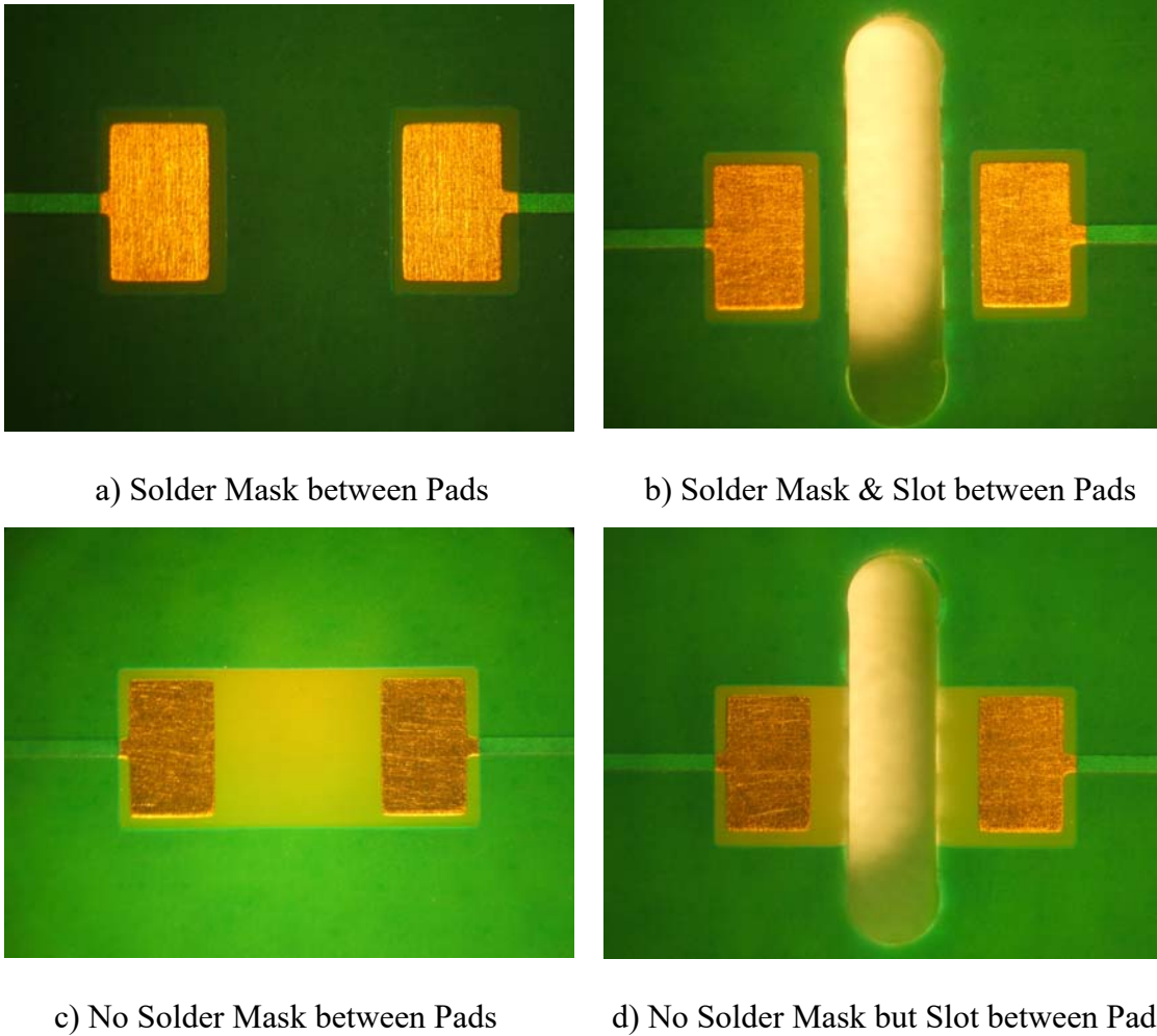
Figure 3. Evaluation Board SMT Pad Variations
