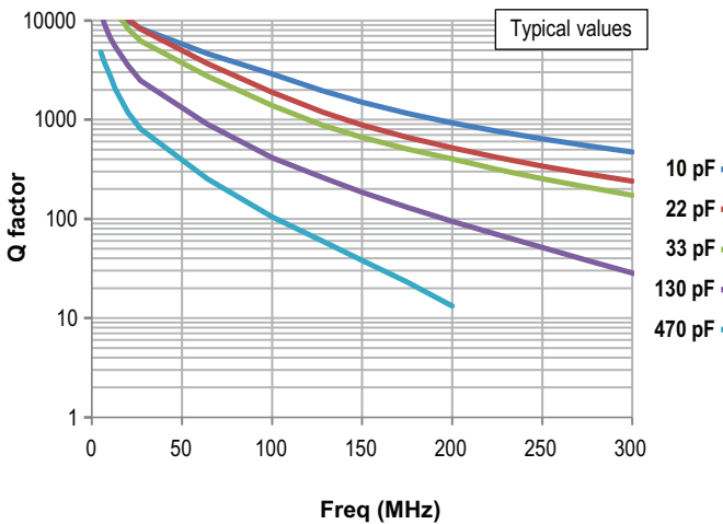
2525 - Q factor
