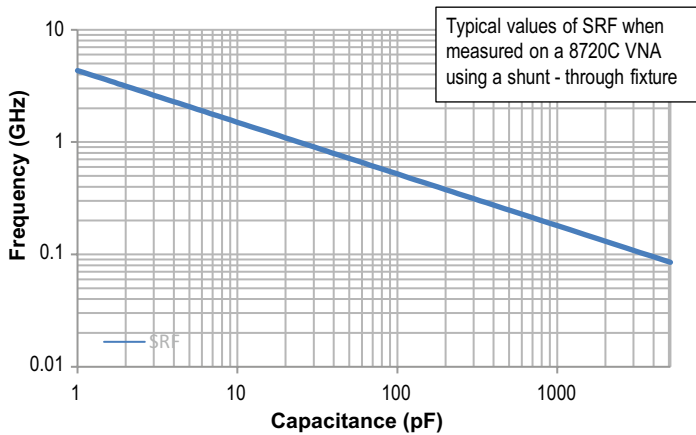
3838 - Resonant Frequency
