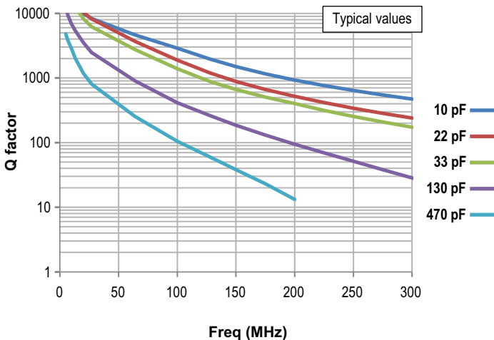
2525 - Q factor
